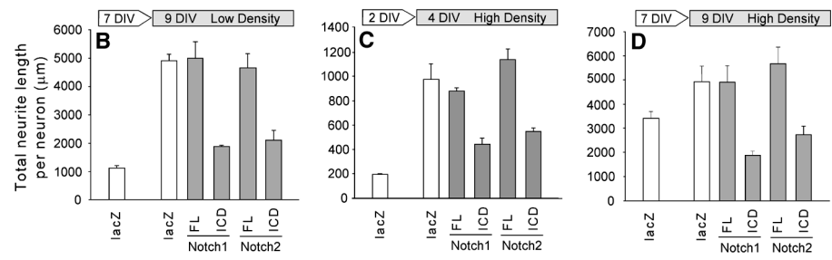
Fig. 3. Human Notch ICD is localized to nuclei and inhibits neurite growth. (A) Confocal images of neurons transfected with human Notch constructs. Scale bar, 12 \mu\text{m} . (B) Total neurite length per neuron in LD cultures at 7 DIV was longer than at 9 DIV ( P = 0.000003 ). Notch FL did not significantly affect neurite growth ( P > 0.61 ). Notch ICD inhibited neurite growth ( P \leq 0.0001 ). (C) In HD cultures, 4 DIV neurons had greater total neurite length than 2 DIV neurons ( P = 0.003 ). Notch FL did not significantly affect neurite growth ( P > 0.35 ). Notch ICD inhibited neurite growth ( P \leq 0.01 ). (D) Total neurite lengths per neuron in HD cultures at 7 and 9 DIV were not significantly different ( P = 0.09 ). Notch FL did not significantly affect the total neurite length ( P > 0.47 ). Notch1 ICD caused neurite retraction in 7 DIV neurons ( P = 0.0037 ). Notch2 ICD inhibited the neurite growth ( P = 0.017 ) but did not cause significant retraction of neurites ( P = 0.19 ) in 7 DIV cultures. Data in (B) to (D) are shown as means \pm SEM ( n \geq 5 trials).
