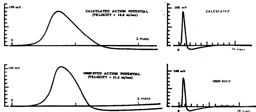
Fig. 9. Propagated action potentials. Top, computed; bottom, observed. Temperature, 18.5°C. From ref. 8.
