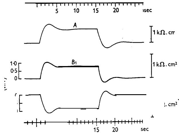
Fig. 14. Responses of the membrane to a constant current, uniformly applied. (A) computed; (B 1 ) and (B 2 ) observed, for currents of +1.49 \mu\text{A}/\text{cm}^2 and -1.49 \mu\text{A}/\text{cm}^2 respectively. 19°C. From ref. 8.
