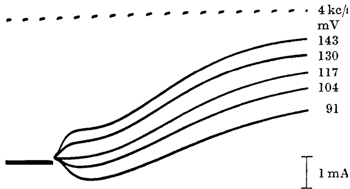
Fig. 3. Membrane currents when the internal potential is raised to values comparable to the peak of an action potential. Axon in sea water; temperature 3.5°C; outward current upwards. The records for 91 and 104 mV displacement of membrane potential show a phase of inward current, while those at 130 and 143 mV show an early hump in the outward current. The record at 117 mV shows neither, and it is therefore taken to be very close to the sodium equilibrium potential, at which the current carried by sodium is zero.
