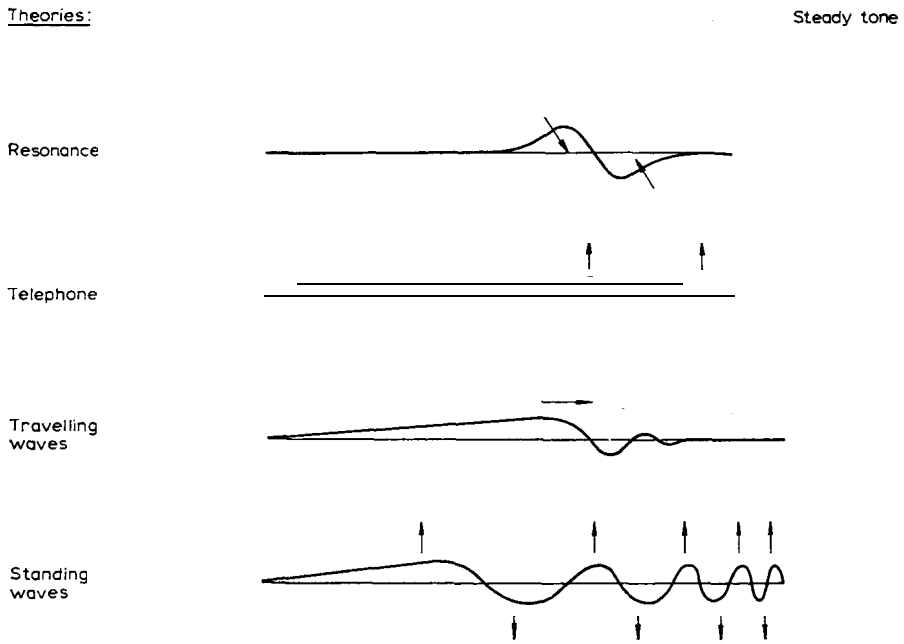
Fig. 22. All the different hearing theories form one family of vibration patterns, differing only in the stiffness of the membrane.
