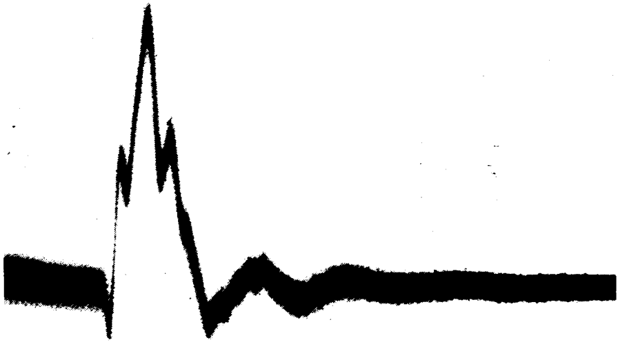
Fig. 12. Vibration of the eardrum after exposure to a very short click.
