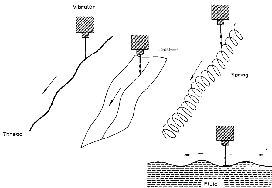
Fig. 15. Travelling waves observed on different objects brought in contact with a vibrator.
