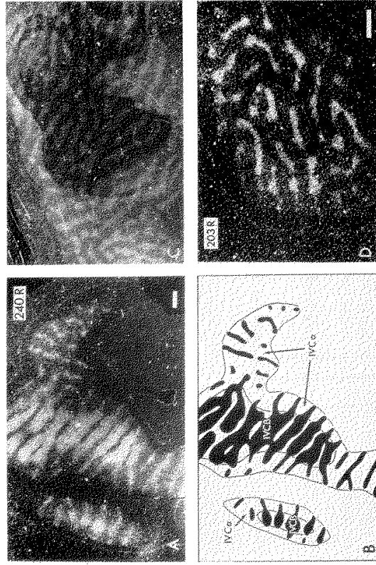
Fig. 9. Effect of reversed suture at various ages on the labelling pattern of geniculate terminals in layer IVC.
