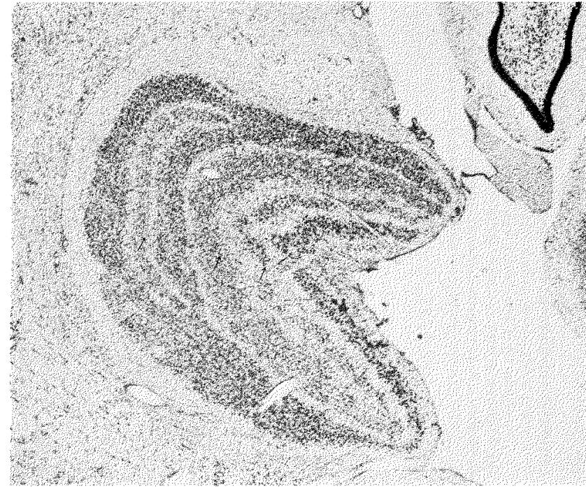
Fig. 2. Coronal section through the right lateral geniculate nucleus of the monkey with right eye closed at 2 weeks for 18 months (fig. 1, right). Note the atrophy in the layers receiving input from the deprived eye (indicated by arrows). Stained with cresyl violet; frozen section. 13
