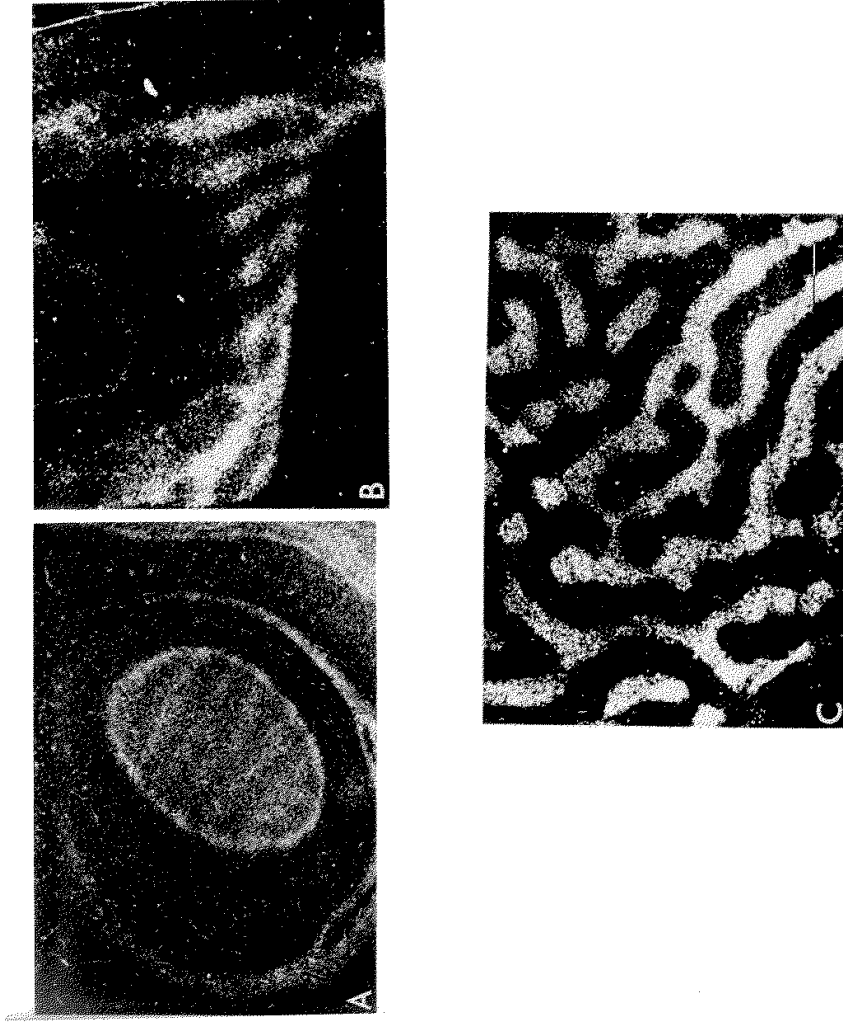
Fig. 13. Darkfield autoradiographs of geniculate afferent terminals in the striate cortex of normal neonatal monkeys in which the right eye had been injected with a radioactive tracer 1–2 weeks earlier. 15
